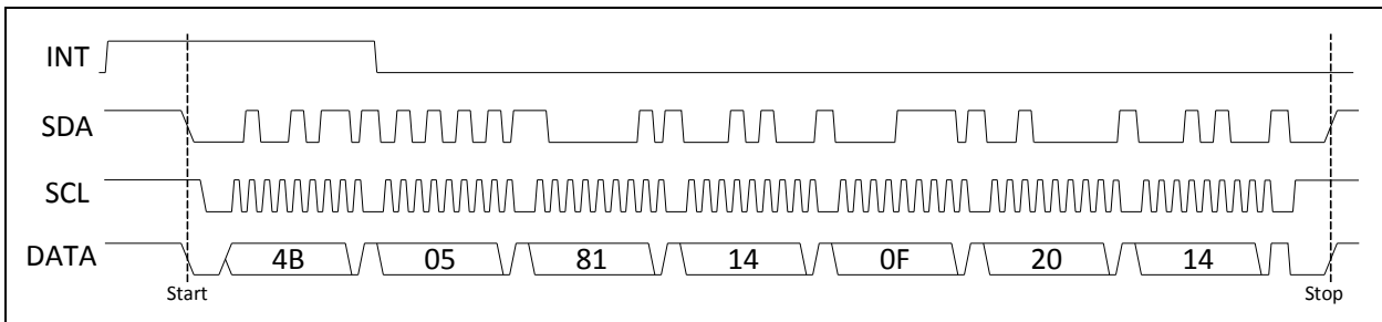
FIGURE 5-8: I 2 C™ TOUCH PACKET READ
