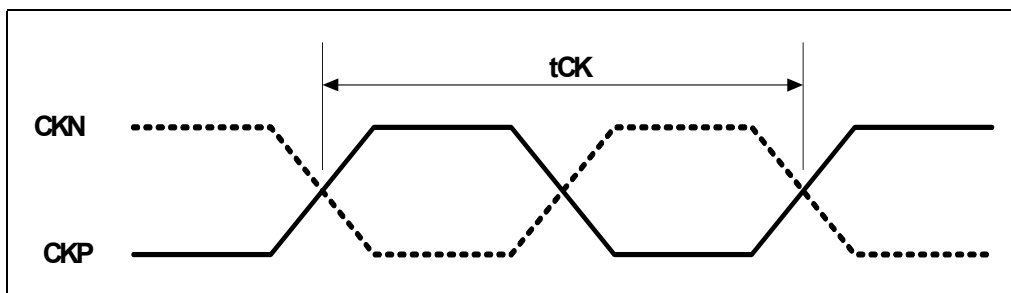
Figure 27. DDR3L Clock Cycle Time
