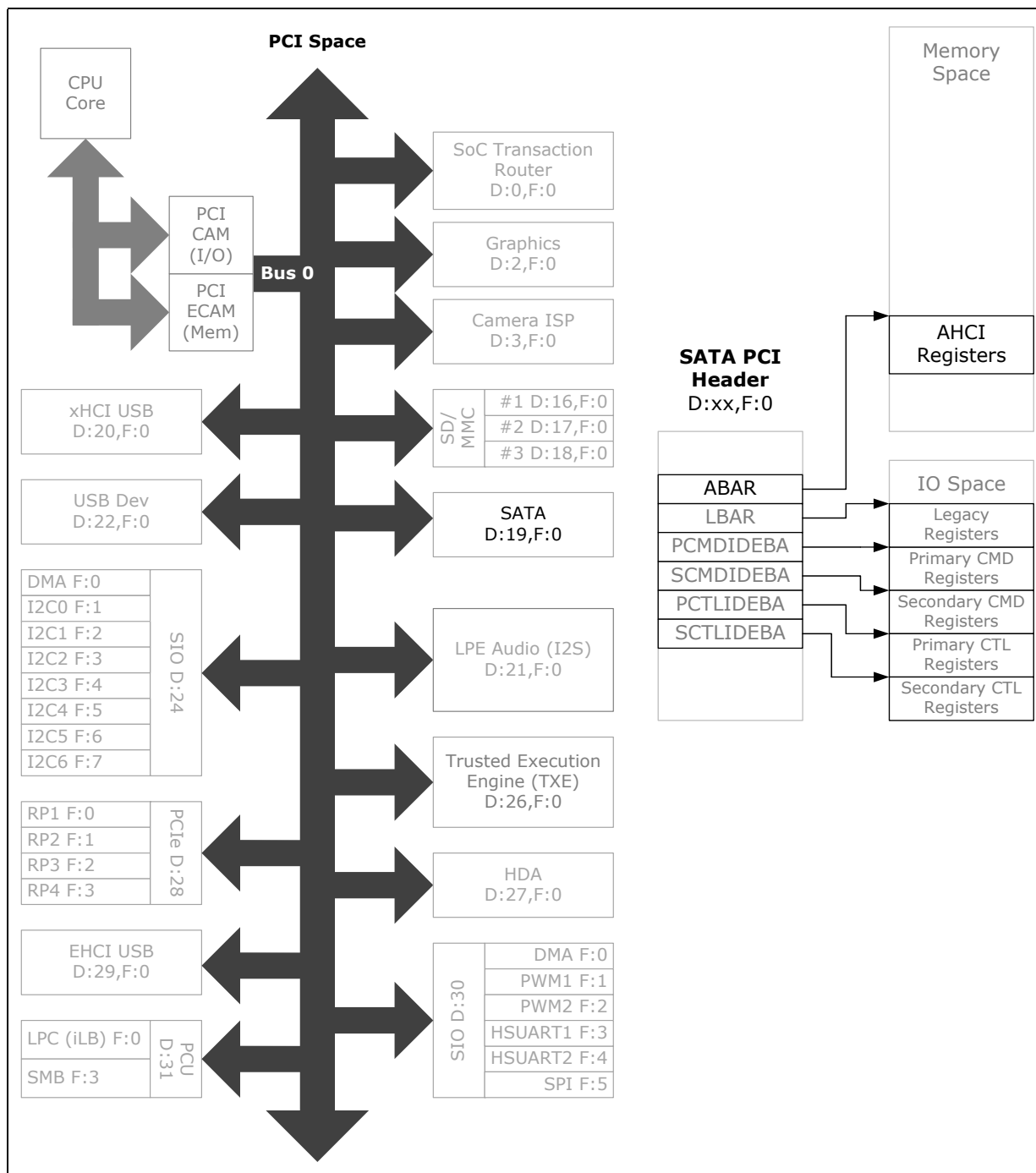
Figure 102.SATA Register Map
