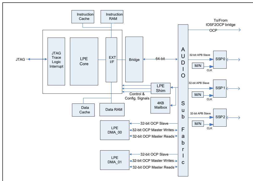
Figure 106. Audio Cluster Block Diagram
