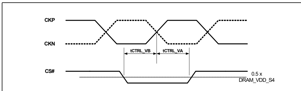
Figure 26. DDR3L ODT Valid before CK Rising Edge
