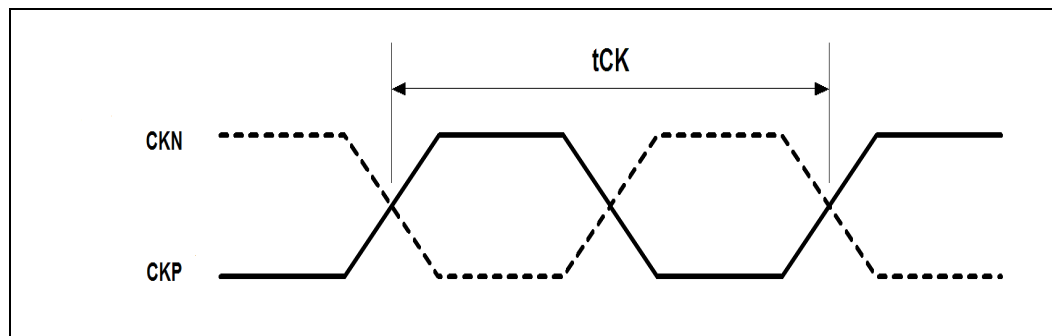
Figure 81. Clock Timing
