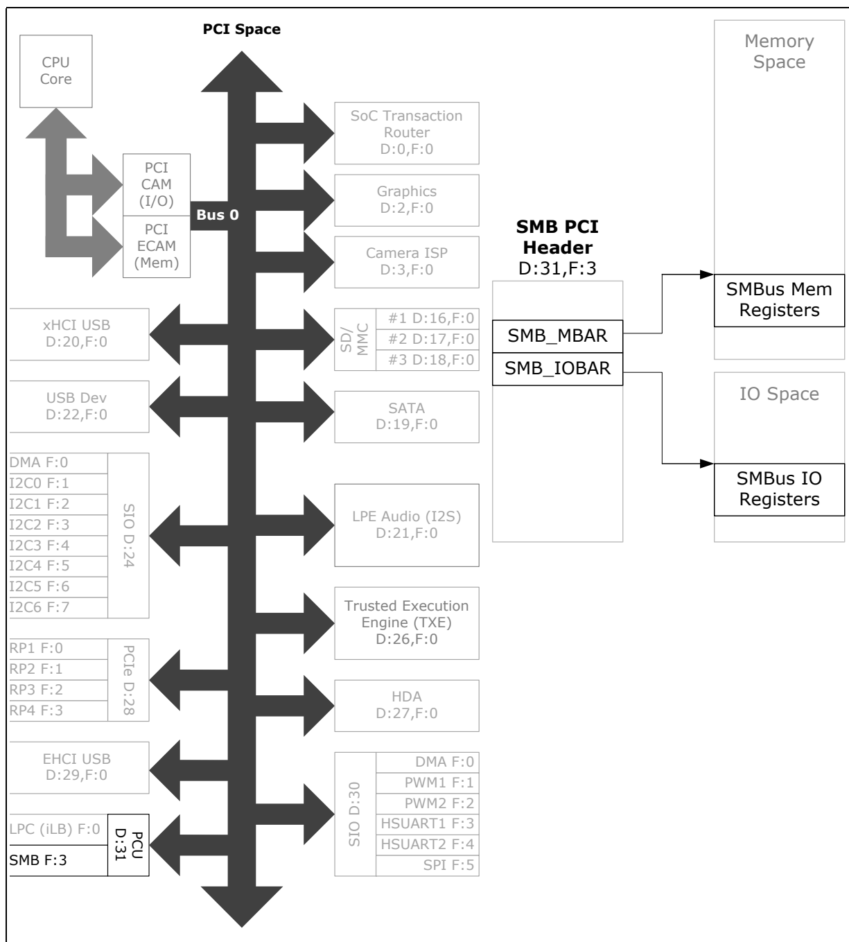
Figure 134.PCU - SMBus Register Map
