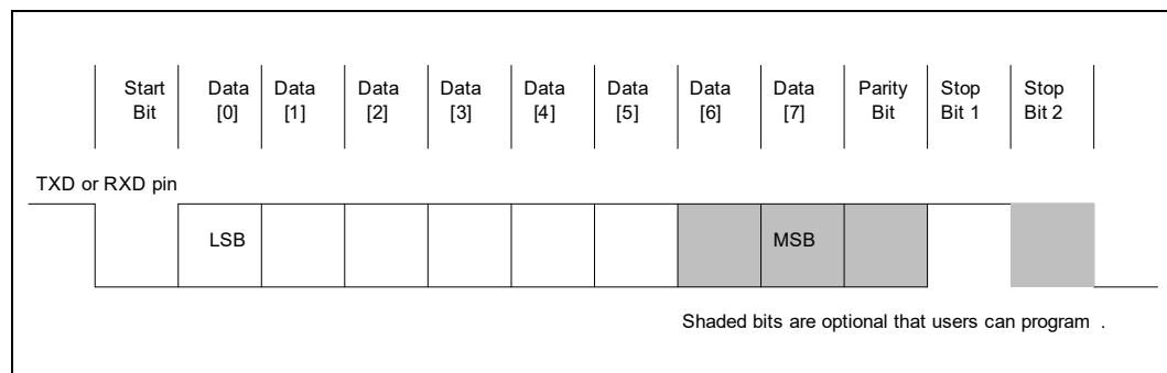
Figure 126. UART Data Transfer Flow
