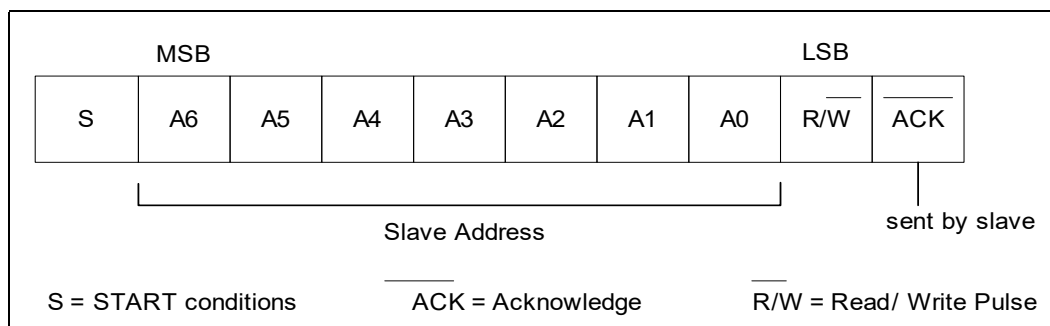
Figure 120. Seven-Bit Address Format
