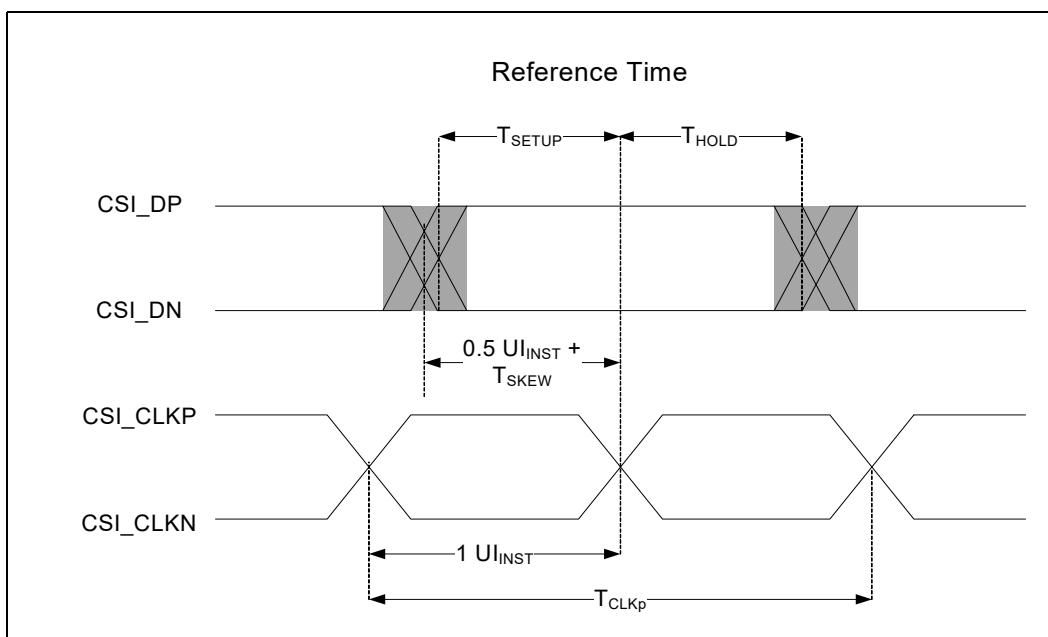
Figure 37. MIPI-CSI-2 Data to Clock Timing Definitions
