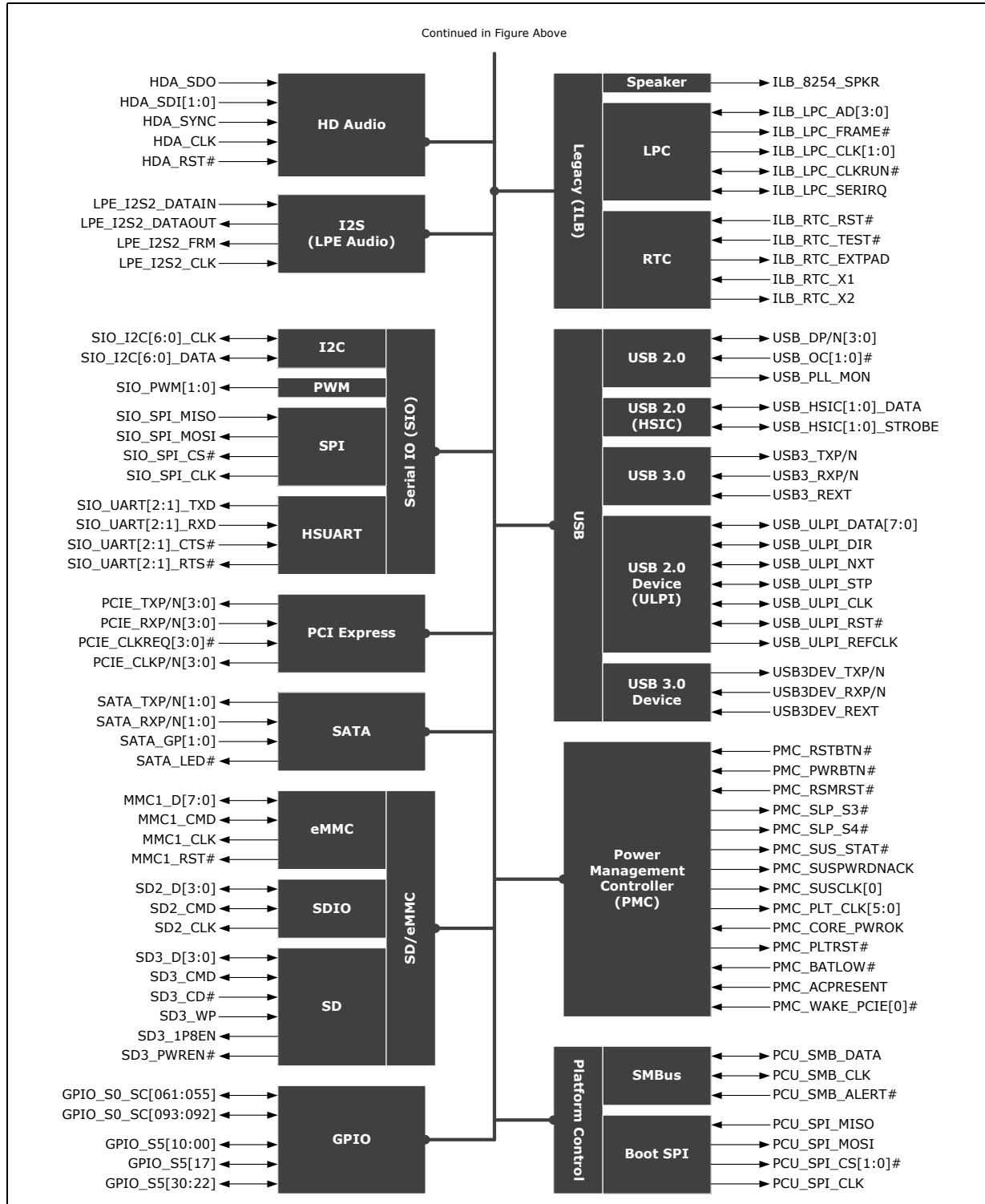
Figure 3. Signals (2 of 2)
