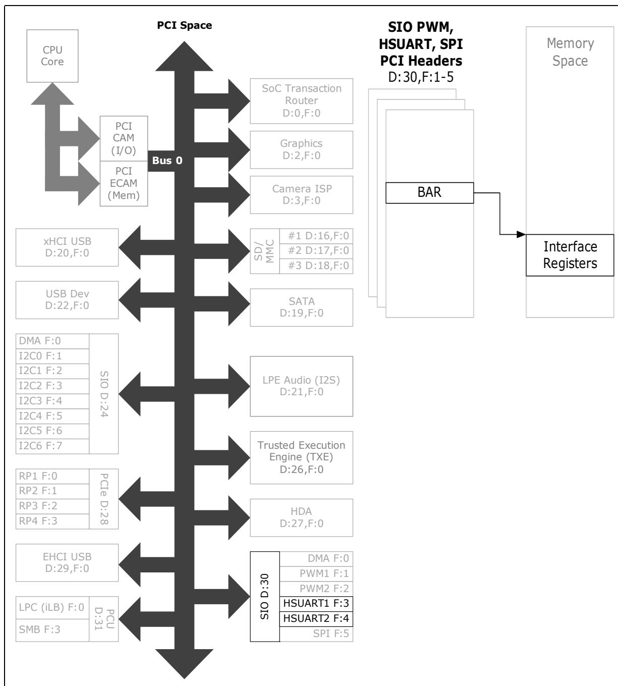
Figure 127.SIO - HSUART Register Map
