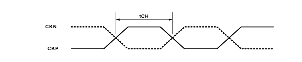
Figure 30. DDR3L CK Low Time
