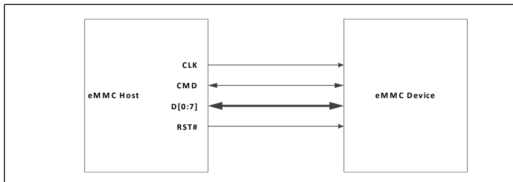
Figure 100.eMMC Interface
