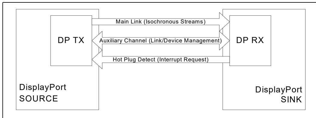
Figure 92. DisplayPort* Overview
