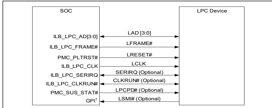
Figure 135. LPC Interface Diagram
