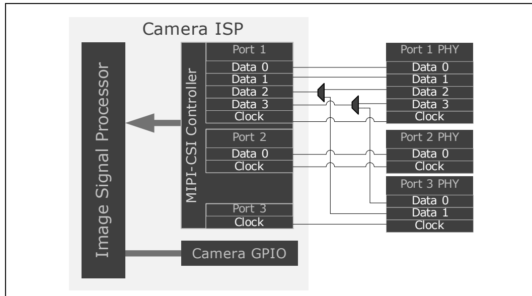
Figure 94. Camera Connectivity
