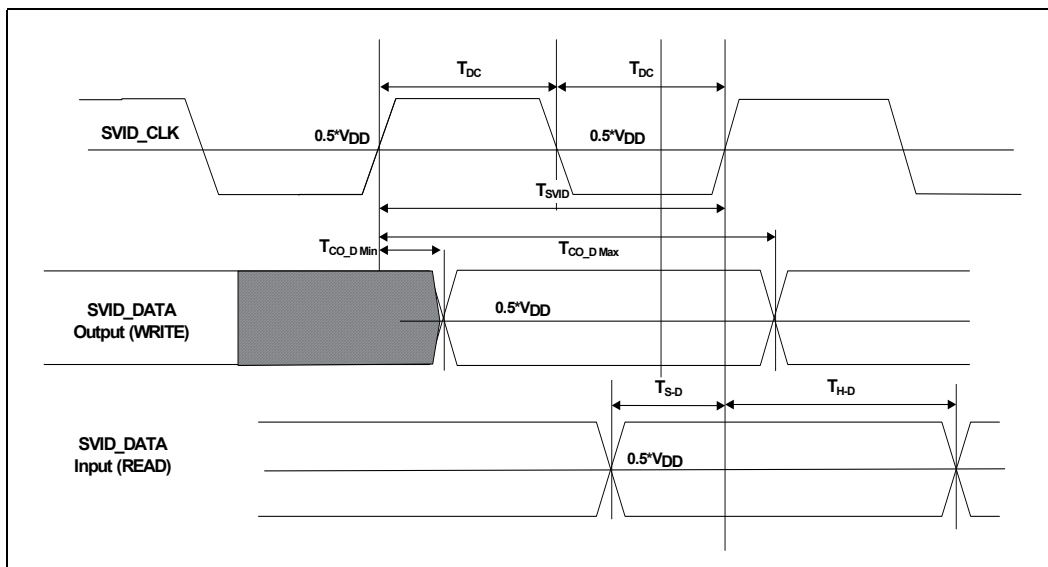
Figure 18. SVID Timing Diagram
