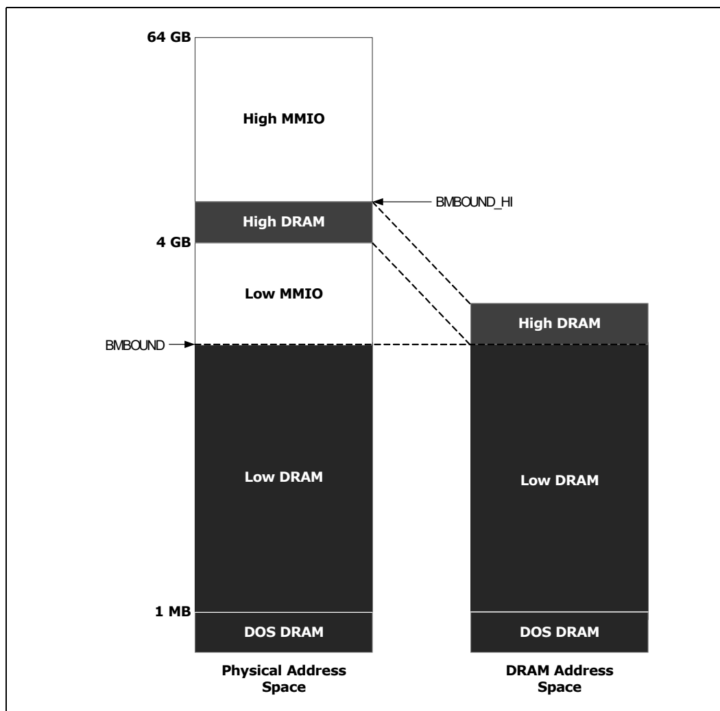
Figure 4. Physical Address Space - DRAM & MMIO
