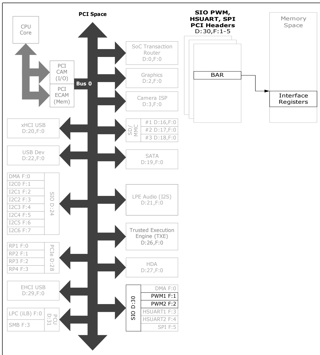
Figure 130.SIO - PWM Register Map
