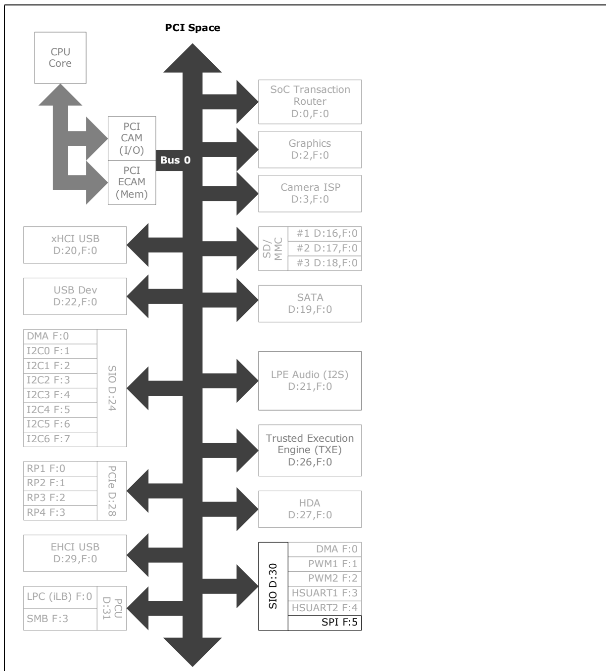
Figure 117.SIO - SPI Register Map
