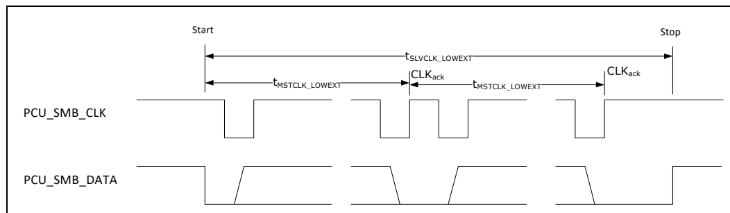
Figure 69. SMBus Timeout
