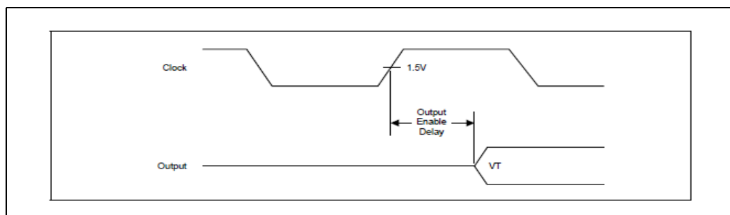
Figure 71. Output Enable Delay
