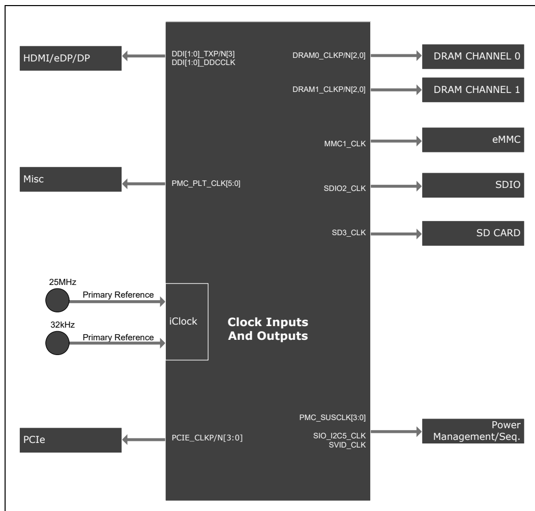
Figure 9. Clocking Example
