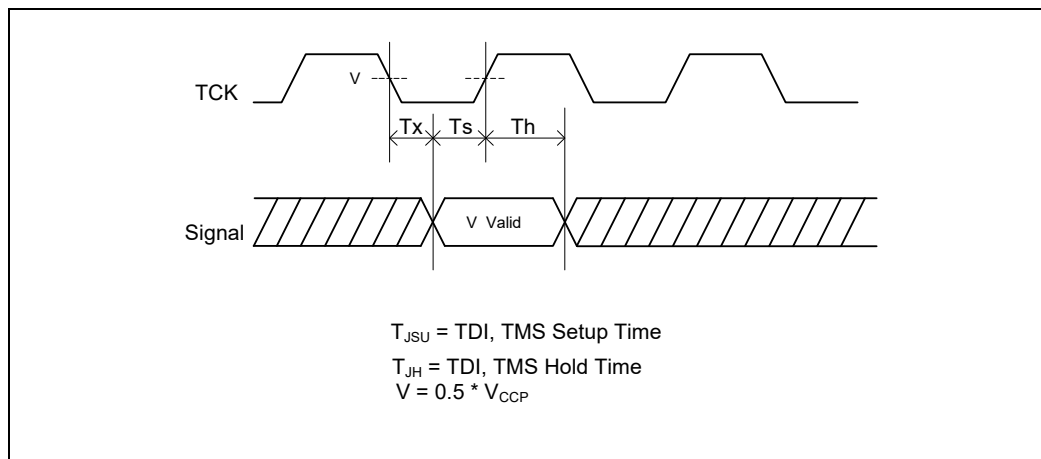
Figure 78. TAP Valid Delay Timing Waveform
