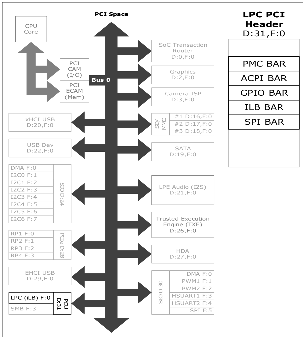
Figure 136. PCU – iLB – LPC Register Map
