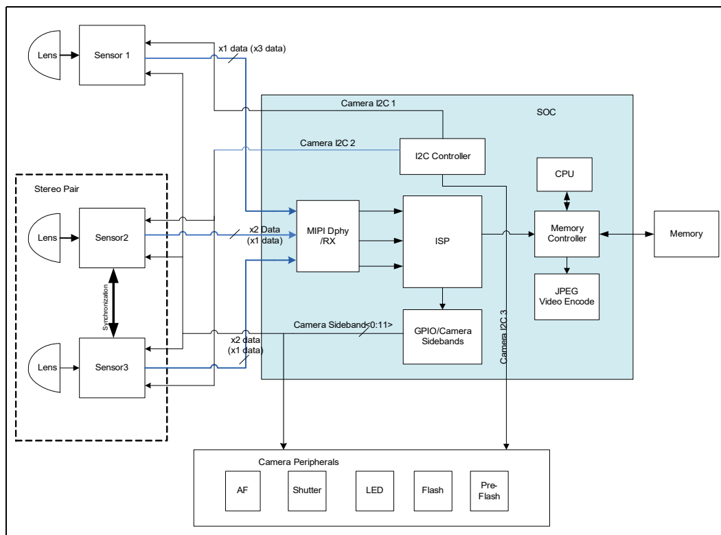
Figure 95. Image Processing Components
