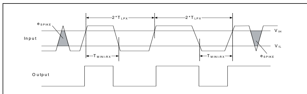
Figure 35. Input Glitch Rejection of Low-Power Receivers
