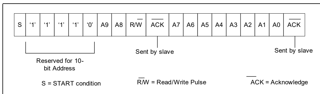
Figure 121. Ten-Bit Address Format
