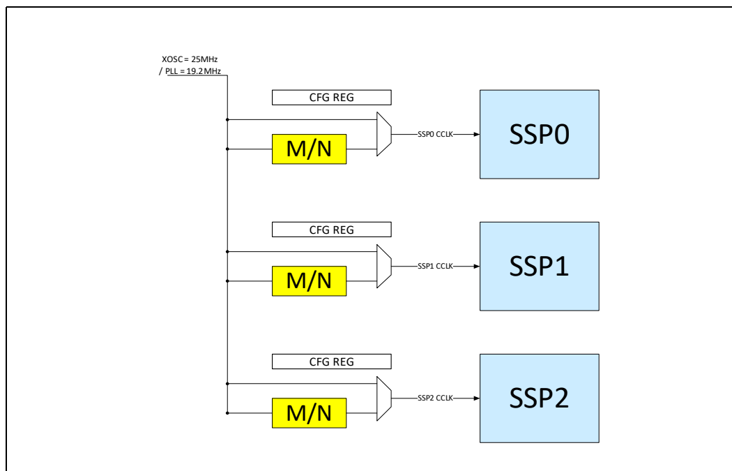
Figure 108.SSP CCLK Structure
