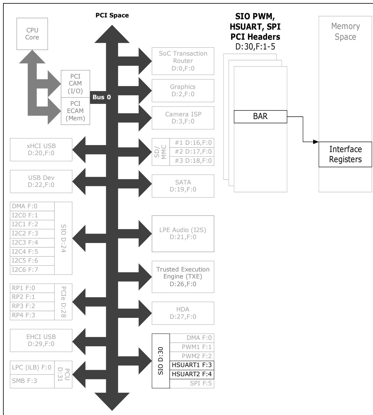
Figure 133.SIO - HSUART Register Map
