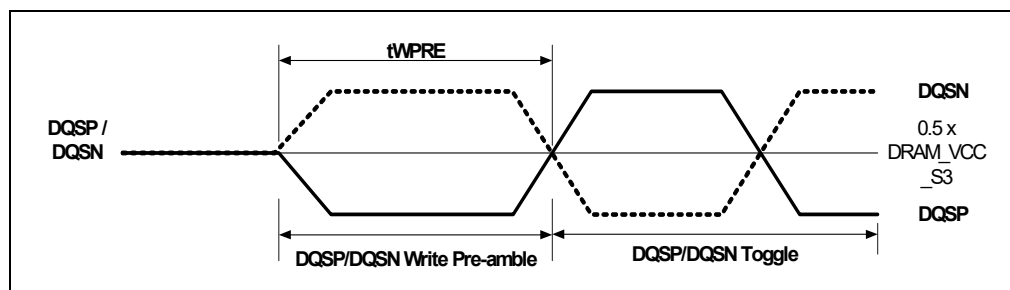
Figure 22. DDR3L Write Post-amble Duration
