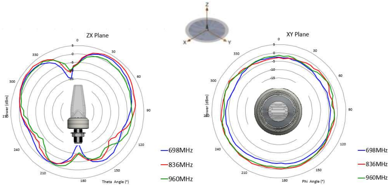
Elevation Plane
