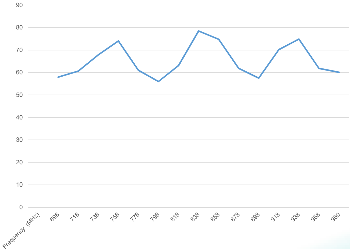
ICEFIN698/960NMO Efficiency (%)
