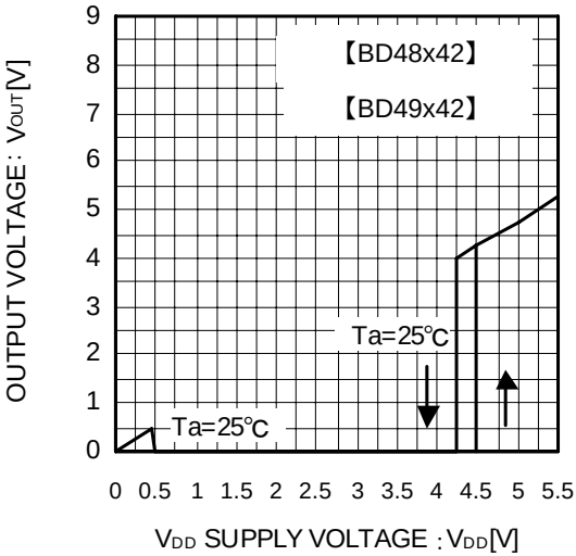
Fig.6 I/O Characteristics
