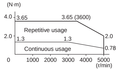
R88M-GP40030H/T (400 W)
