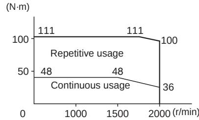
R88M-G7K515T (7.5 kW)
