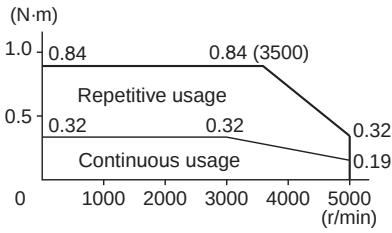
R88M-GP10030L/S (100 W)
