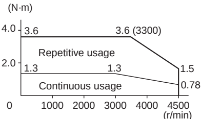
R88M-GP40030L/S (400 W)
