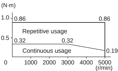
R88M-GP10030H/T (100 W)
