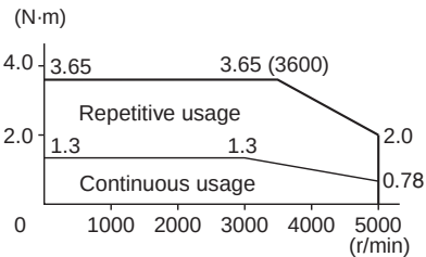
R88M-GP40030H/T (400 W)
