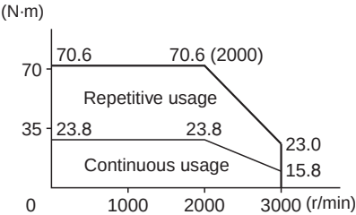
R88M-G5K020T (5 kW)
