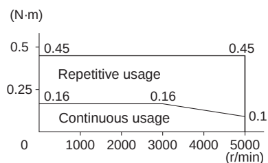
R88M-G05030H/T (50 W)
