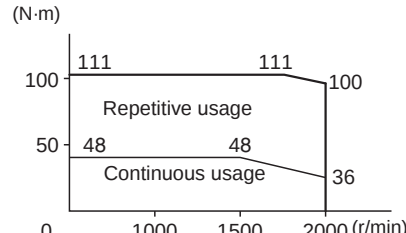
R88M-G7K515T (7.5 kW)
