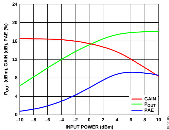
Figure 24. Power Compression at 2 GHz
