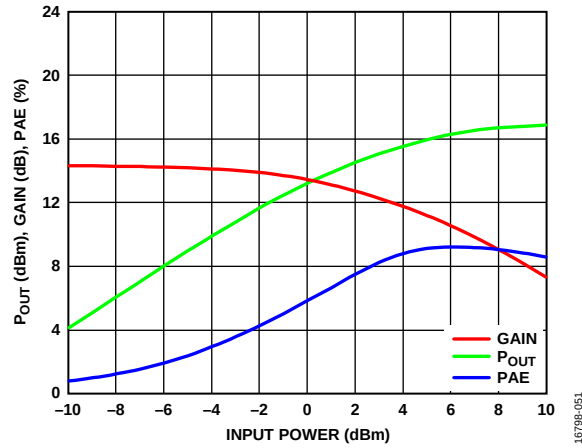
Figure 25. Power Compression at 10 GHz
