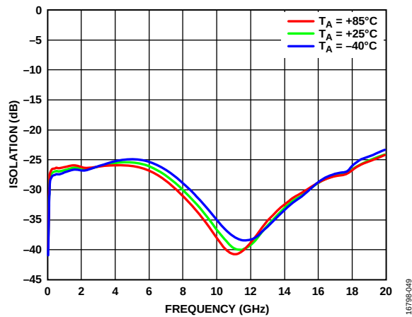
Figure 23. Reverse Isolation vs. Temperature
