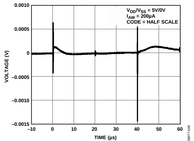
Figure 35. Digital Feedthrough
