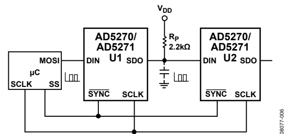
Figure 44. Daisy-Chain Configuration Using SDO
