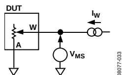
Figure 39. Resistor Position Nonlinearity Error (Rheostat Operation; R-INL, R-DNL)
