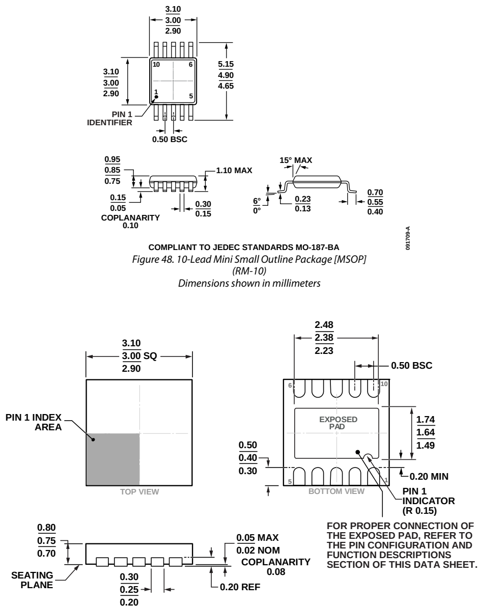
Figure 49. 10-Lead Frame Chip Scale Package [LFCSF_WD] 3 mm × 3 mm Body, Very Thin, Dual Lead (CP-10-9)
