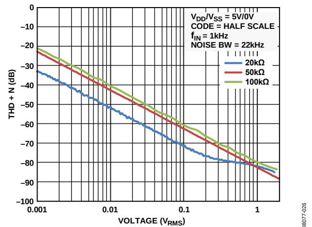
Figure 34. THD + N vs. Amplitude
