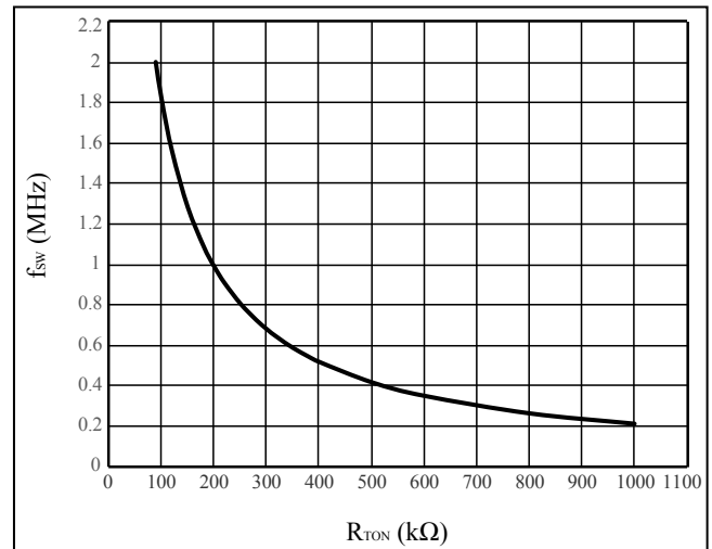
Figure 29 Operating Frequency vs. R TON Resistance
