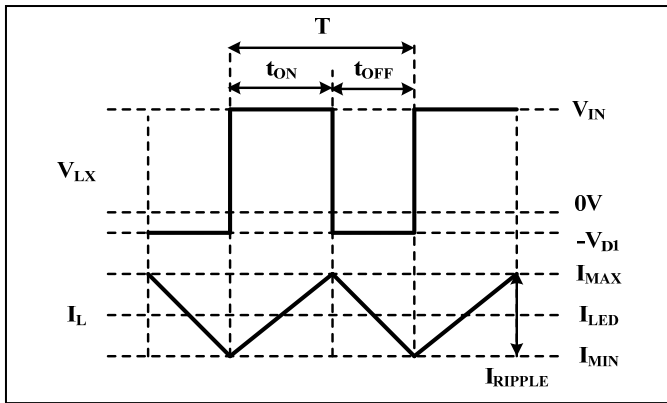
Figure 30 Operating Waveform
