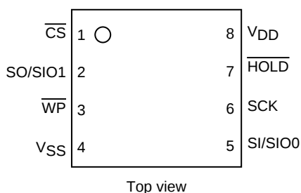
Figure 1 Pin Assignments
