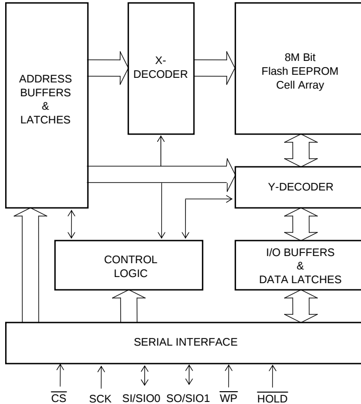
Figure 2 Block Diagram
