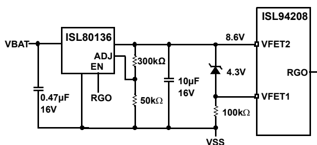
FIGURE 31. ISL94208 EXAMPLE ALTERNATIVE VFET POWER SUPPLY
