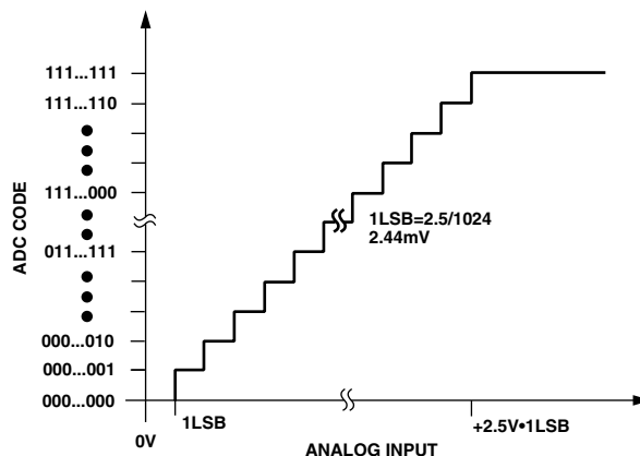
Figure 10. ADC Transfer Function
