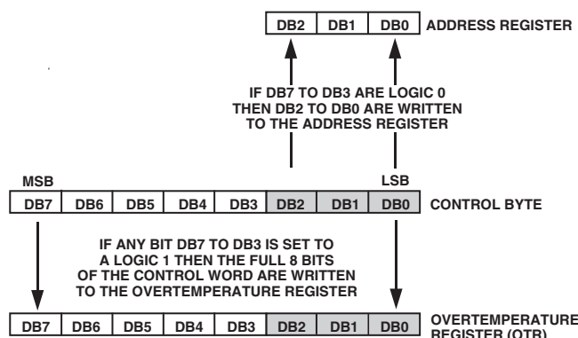
Figure 4. Address and Overtemperature Register Selection
