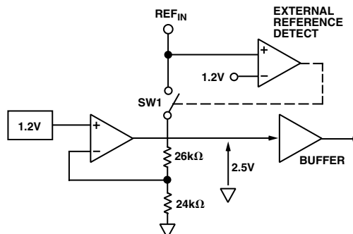
Figure 9. On-Chip Reference
