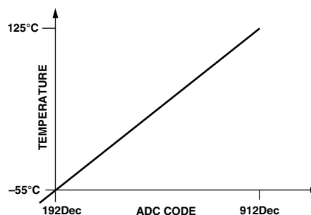
Figure 11. Temperature Sensor Transfer Characteristic
