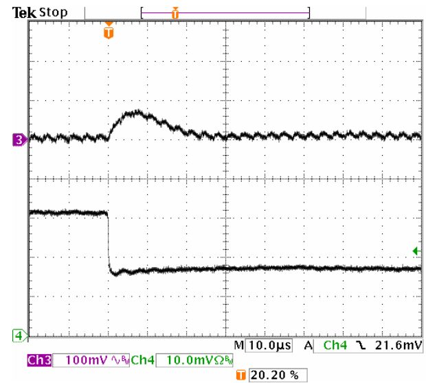
Fig-1.0V-7: Output voltage response for V_{out}=1.0V to positive load current step-change from 3A to 1.5A with slew rate of -5A/\mu s at V_{in}=5.0V . C_o=47\mu F \times 2 ceramic. Top trace: output voltage (100mV/div.) Bottom trace: load current (1A/div.) Time scale: 10μs/div.
