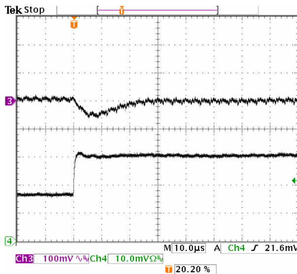
Fig-1.0V-6: Output voltage response for V_{out}=1.0V to positive load current step-change from 1.5A to 3A with slew rate of 5A/\mu s at V_{in}=5.0V . C_o=47\mu F \times 2 ceramic. Top trace: output voltage (100mV/div.) Bottom trace: load current (1A/div.) Time scale: 10μs/div.
