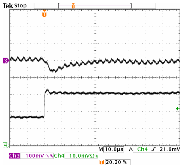
Fig-2.5V-6: Output voltage response for V_{out}=2.5V to positive load current step-change from 1.5A to 3A with slew rate of 5A/\mu s at V_{in}=5.0V . C_o=47\mu F \times 2 ceramic. Top trace: output voltage (100mV/div.) Bottom trace: load current (1A/div.) Time scale: 10μs/div.
