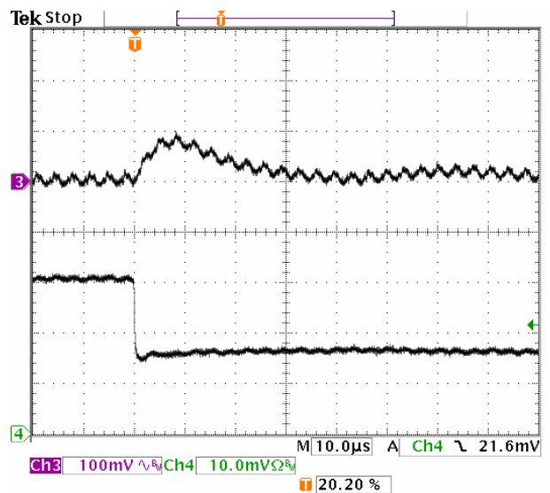
Fig-2.5V-7: Output voltage response for V_{out}=2.5V to positive load current step-change from 3A to 1.5A with slew rate of -5A/\mu s at V_{in}=5.0V . C_o=47\mu F \times 2 ceramic. Top trace: output voltage (100mV/div.) Bottom trace: load current (1A/div.) Time scale: 10μs/div.
