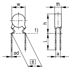
1) Seating plane to IEC 60717 VAR04111-F-E
