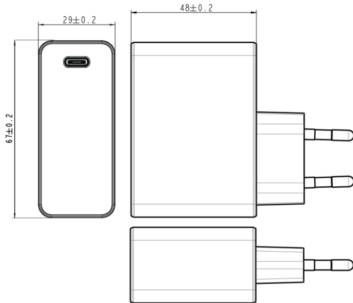
AQ45E-5CKA Dimension Diagram Unit: mm (inch)
