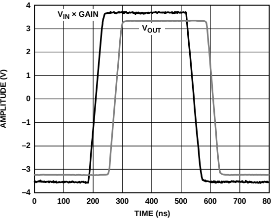
Figure 14. Overdrive Recovery
