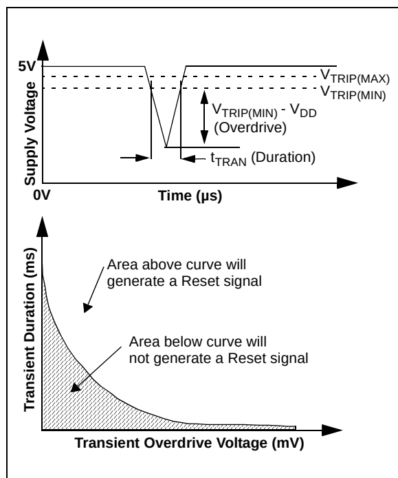
FIGURE 4-9: Example of Typical Transient Duration Waveform.
