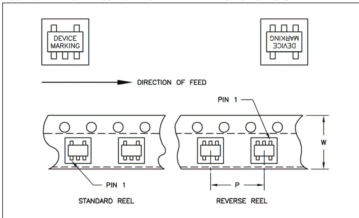
FIGURE 9-2: 5-LEAD SOT-23 DEVICE TAPE AND REEL SPECIFICATIONS
