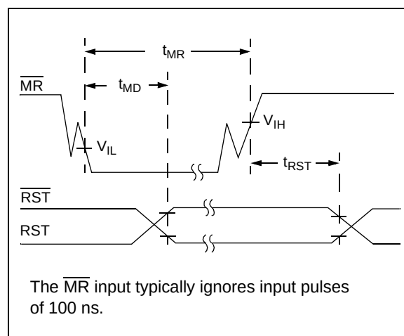
FIGURE 4-11: \overline{MR} Input – Push Button.
