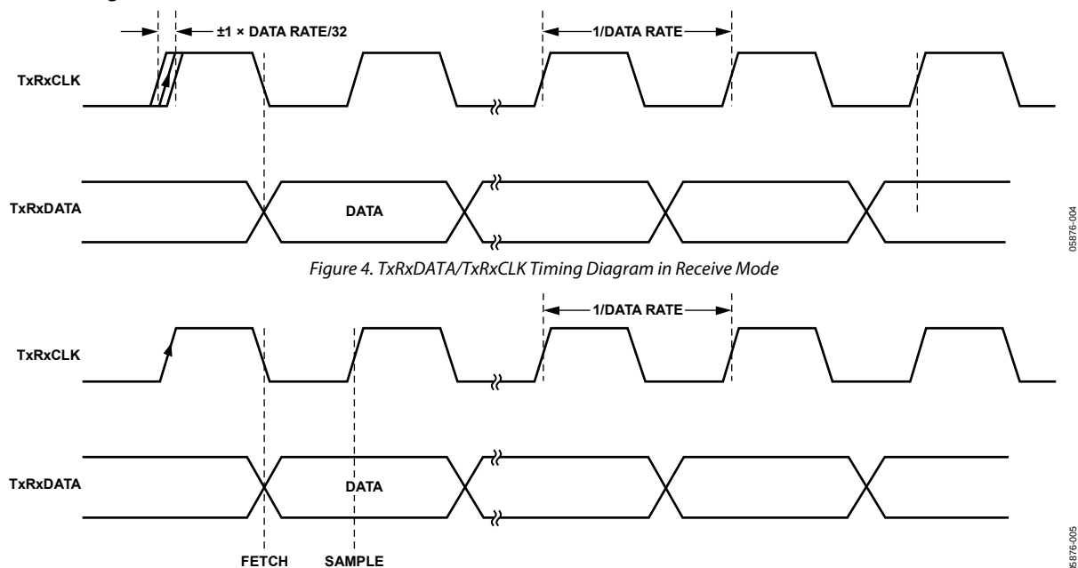
Figure 5. TxRxDATA/TxRxCLK Timing Diagram in Transmit Mode
