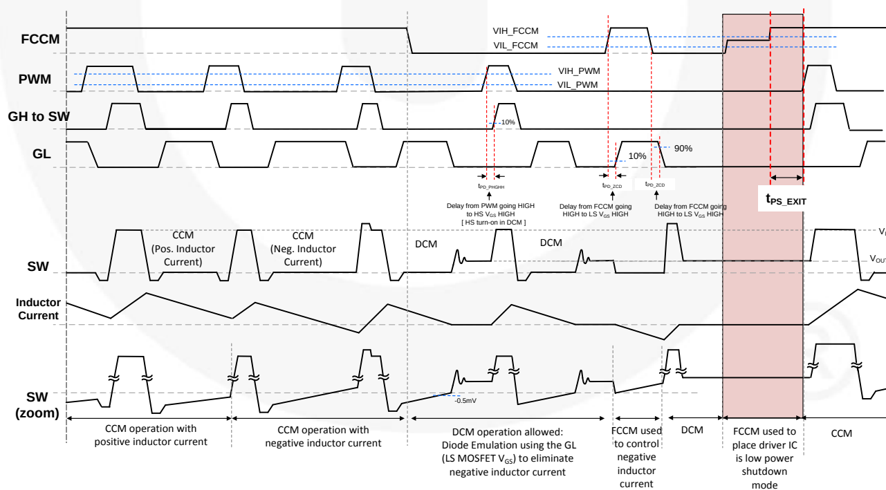
FCCM 3-State Timing Diagram
