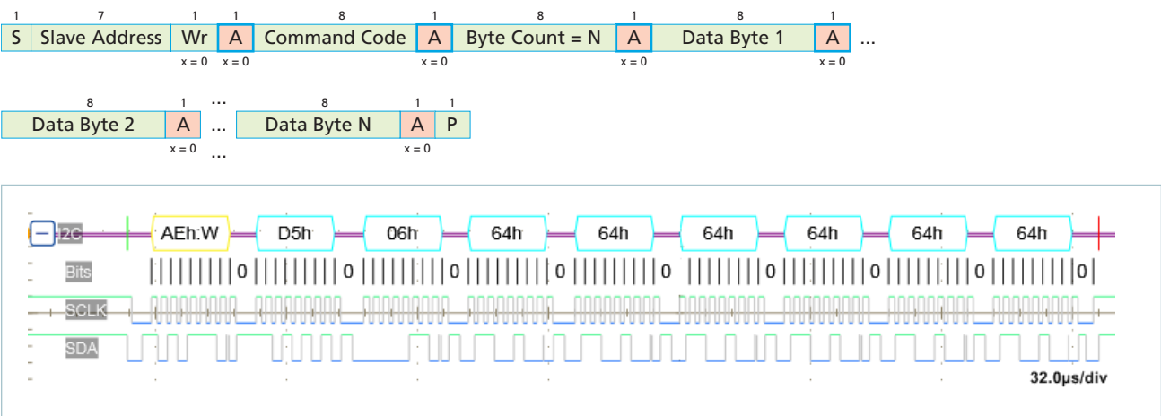
Figure 5 — SET_ALL_THRESHOLDS COMMAND (D5h)_WRITE BLOCK PROTOCOL
