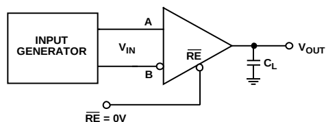
Figure 42. Receiver Propagation Delay/Skew
