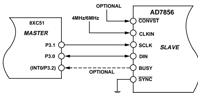
Figure 37. 8XC51/PIC16C42 Interface
