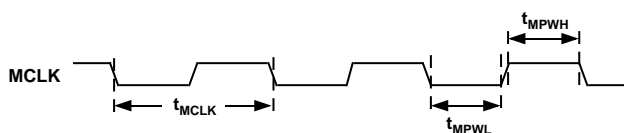
Figure 24. AD1890/AD1891 MCLK Timing
