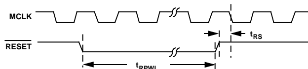
Figure 25. AD1890/AD1891 Reset Timing
