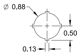
22.5mm Detail
