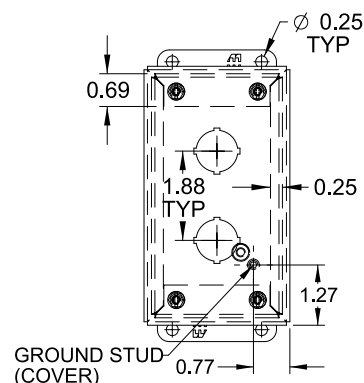
Front View Body Type MPB1 through MPB4 (Not Hinged)
