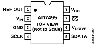
Figure 6. AD7495 SOIC/MSOP Pin Configuration
