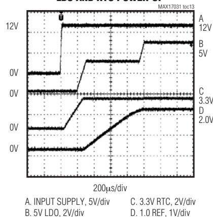
LDO AND RTC POWER-UP
