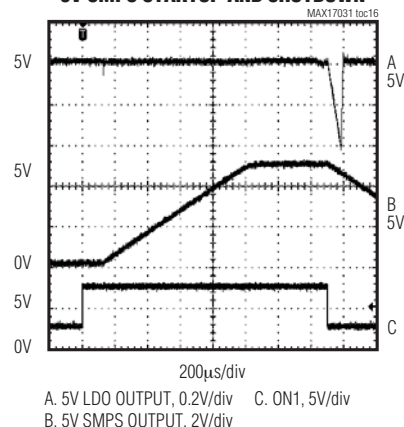
5V SMPS STARTUP AND SHUTDOWN
