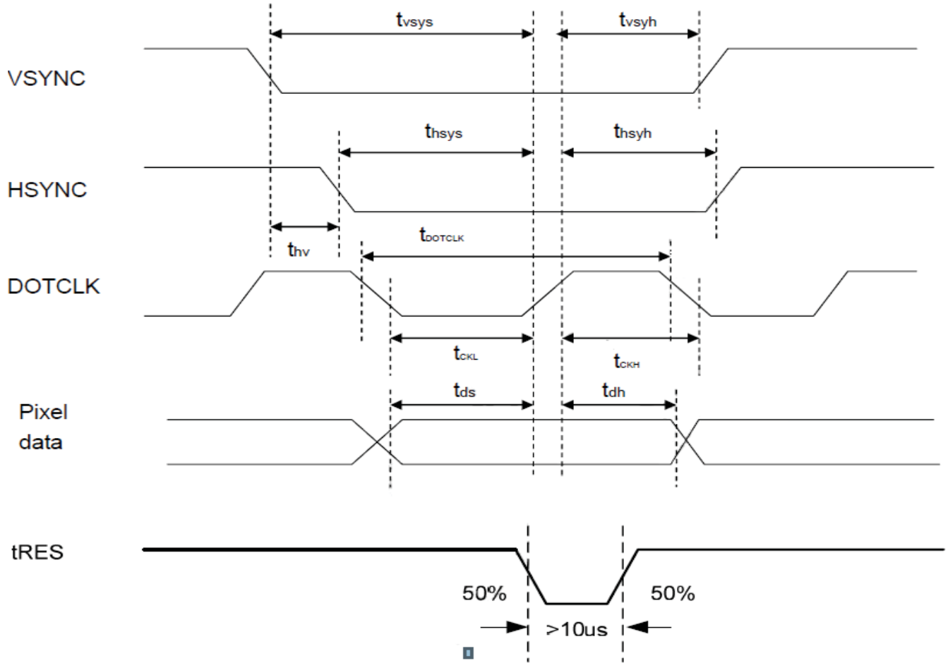
Figure 3: Pixel Timing
