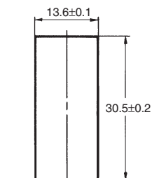
Panel Cutout
