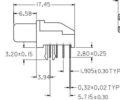
FOR CIRCUIT SIZE 50 ONLY
