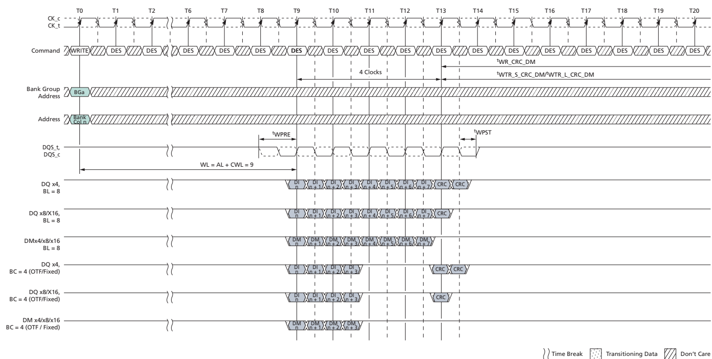
Figure 196: WRITE (BL8/BC4-OTF/Fixed) with 1 st CK Preamble and Write CRC in Same or Different Bank Group
