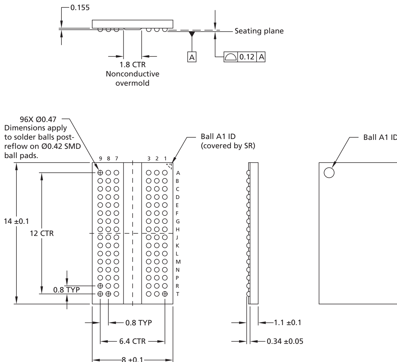
Figure 8: 96-Ball FBGA – x16 (JY)
