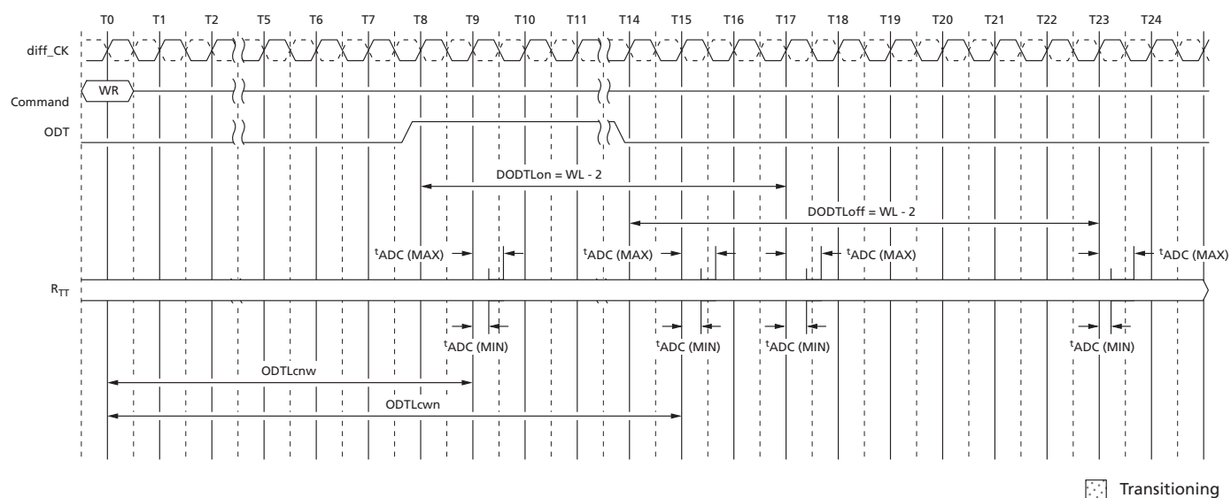
Figure 202: Dynamic ODT (1 st CK Preamble; CL = 14, CWL = 11, BL = 8, AL = 0, CRC Disabled)
