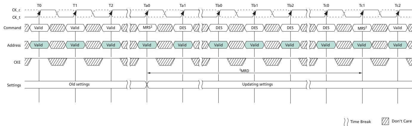
Figure 13: t_{MRD} Timing
