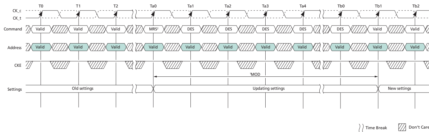
Figure 14: t_{MOD} Timing
