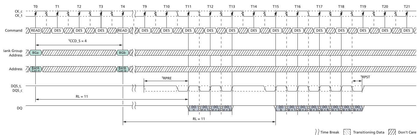
Figure 137: READ (BC4) to READ (BL8) OTF with 2 t CK Preamble in Different Bank Group
