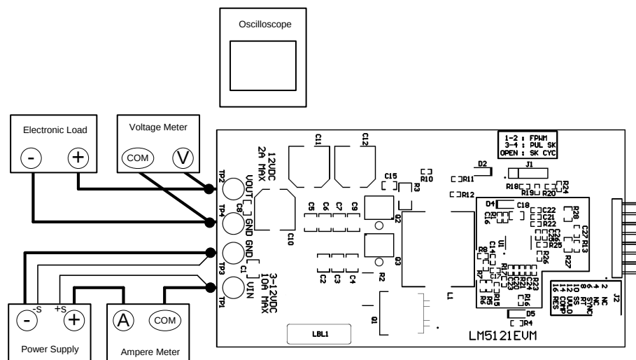
Figure 2. Connection Diagram
