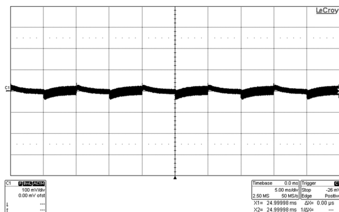
Figure 4. Load Transient
