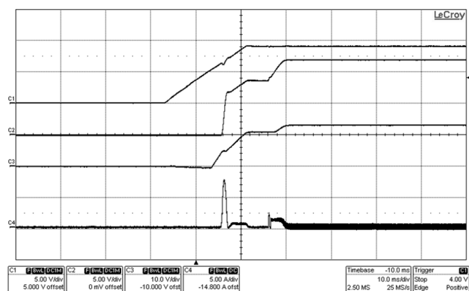
Figure 10. Start-up
