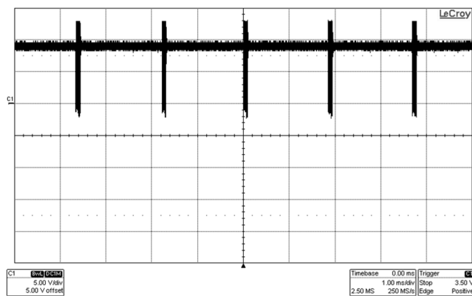
Figure 8. Skip Cycle
