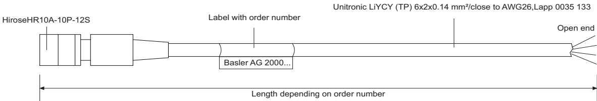
Fig. 1: Cable Overview
