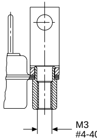
Metal Bracket with Post (1AHN/1A8N)
