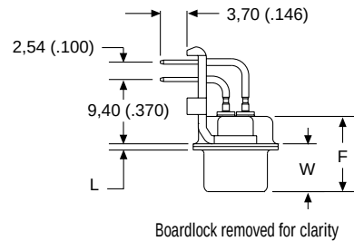
Boardlock removed for clarity
