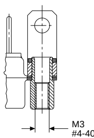
Plastic Bracket with Post (1APN/1A6N)
