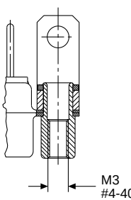
Plastic Bracket with Post (1APN/1A6N)
