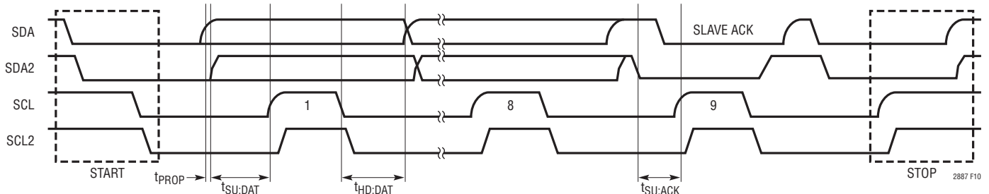
Figure 10. I 2 C Timing Diagram
