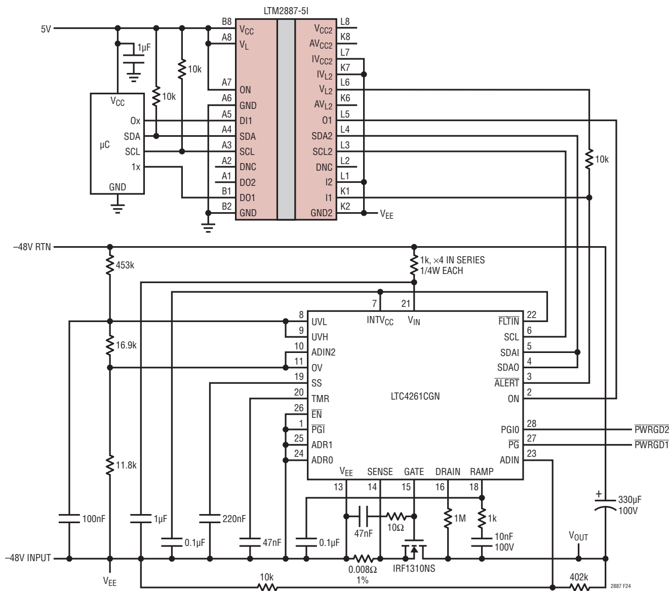
Figure 24. -48V, 200W Hot Swap Controller with Isolated I 2 C Interface
