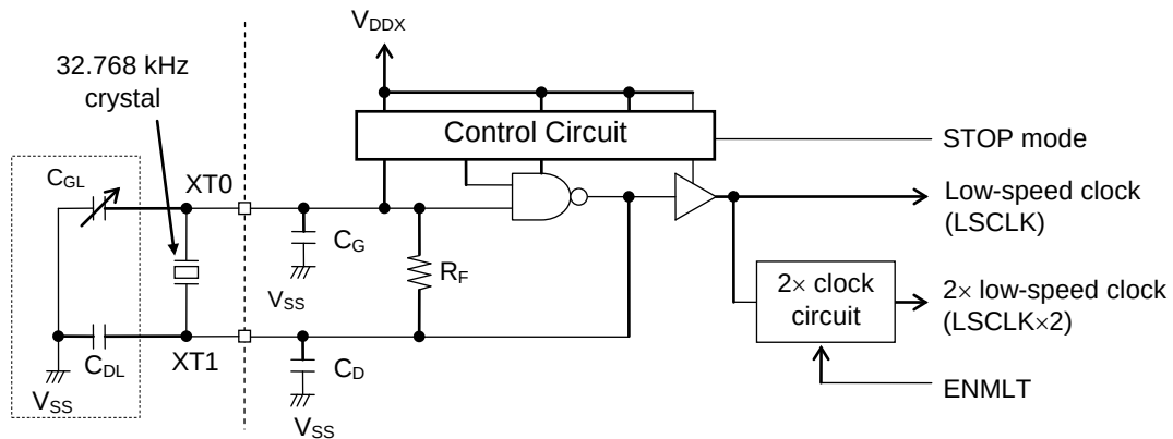
Figure 6-2 Circuit Configuration of 32.768 kHz Crystal Oscillation Mode
