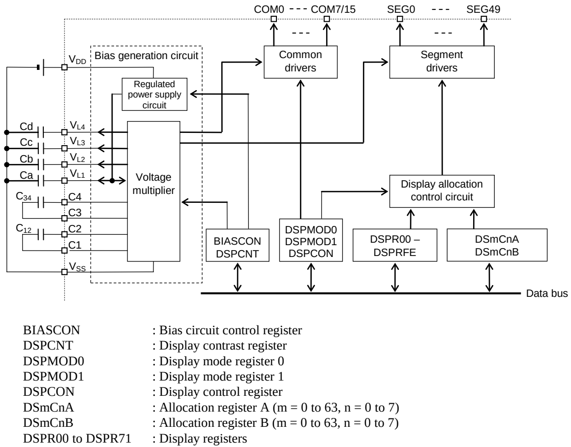
Figure 26-4 Configuration of LCD Drivers and Bias Generation Circuit
