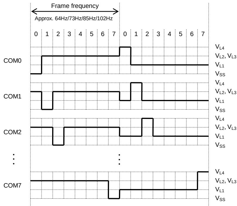
Figure 26-9 (1) Common Output Waveforms for 1/8 Duty and 1/3 Bias
