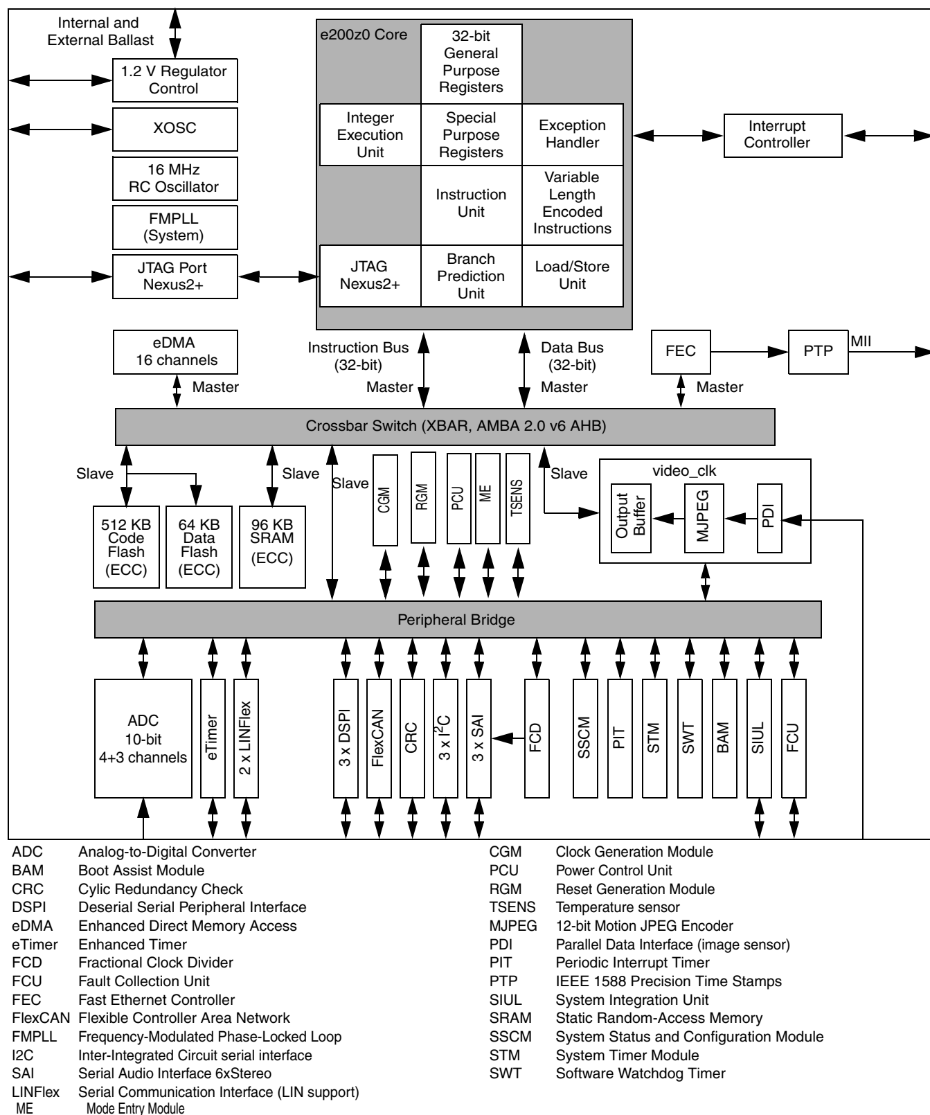
Figure 1. MPC5604E block diagram
