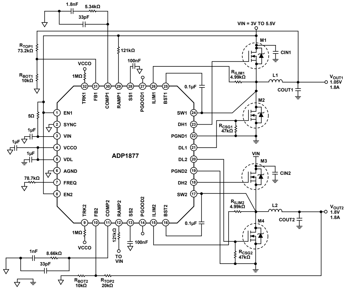
Figure 44. Typical Low Current Application with V_{IN} < 5.5\text{ V}
