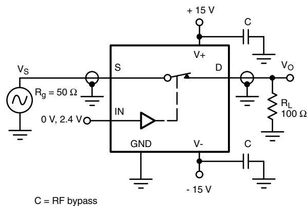
Figure 6. Insertion Loss
