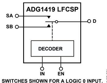
Figure 1. 8-Lead LFCSP (CP-8-4)
