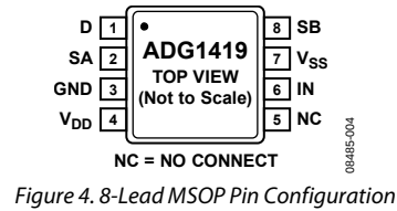
Figure 4. 8-Lead MSOP Pin Configuration
