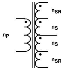
Figure 8. Transformer Schematic
