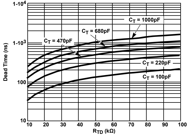
Figure 4. Dead Time vs Capacitance
