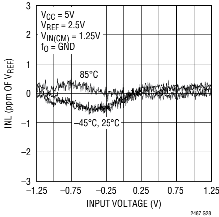
Integral Nonlinearity (2x Speed Mode; V_{CC} = 5V , V_{REF} = 2.5V )
