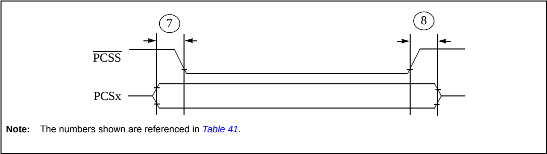
Figure 40. DSPI PCS strobe (PCSS) timing
